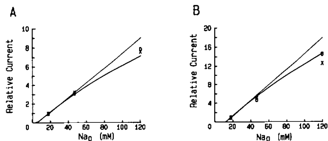
FIGURE 3 Normalized peak I_{Na} of two perfused single Purkinje cells (○, ×) as a function of extracellular permeant ion concentrations of 18, 47, and 121 mM at test potentials of -30 mV (A) and -10 mV (B). The straight lines represent normalized current predicted by ionic independence while the curved lines represent model fits to the data (see text).
