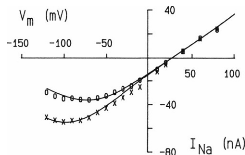
FIGURE 8 Instantaneous current voltage plot in a perfused Purkinje cell with either 3.0 mM (×) or 10.0 mM (○) Ca^{2+} . The lines represent model fits to the data (see text).
