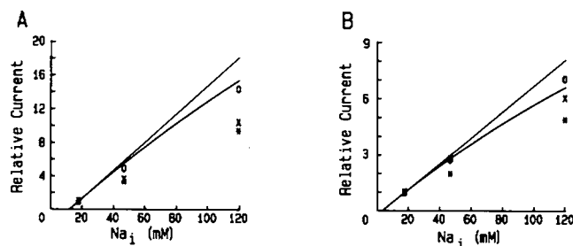
FIGURE 4 Normalized peak I_{Na} of three perfused single Purkinje cells (0, \times , \ast ) as a function of intracellular permeant ion concentrations of 18, 47, and 121 mM at test potentials of +10 mV (A) and +40 mV (B). The straight lines represent normalized current predicted by ionic independence while the curved lines represent model fits to the data (see text).
