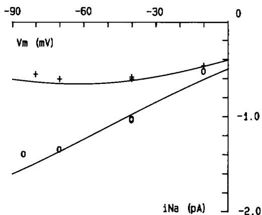
FIGURE 6 Plots of the i/V relationships with 1.0 mM Mg^{2+} and 0 mM (○) or 10 mM (*) Ca^{2+} in the patch pipette. Each point represents the average amplitudes of 34–240 single channel openings. The solid lines are model fits to the data (see text).
