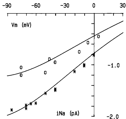
FIGURE 2 Plots of the i/V relationships with 140 mM (○) or 280 mM (×) in the patch pipette. Each point represents the average of 70–420 single channel openings. The solid lines are the model predictions using the parameters from Fig. 9.
